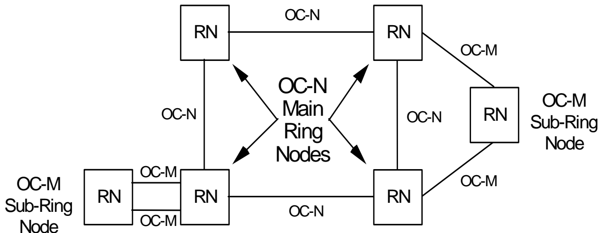
Sub-Ring Nodes, OC-M &lt; OC-N
